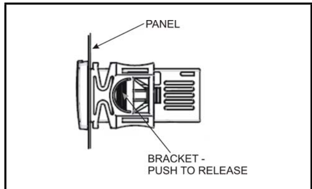
Figure 10-1 - Installation and Mounting of XR75CX-CD
