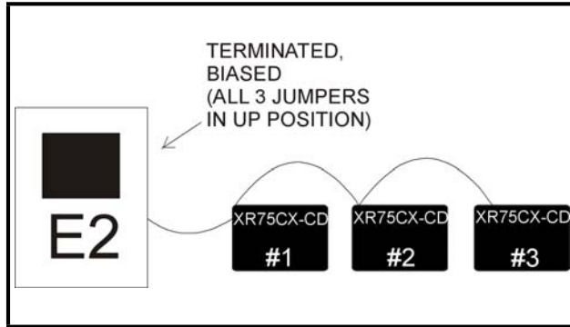
Figure 16-3 - MODBUS Networking
