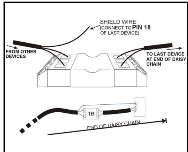
Figure 16-9 - MODBUS Termination Block ( P/N 535-2711 )
