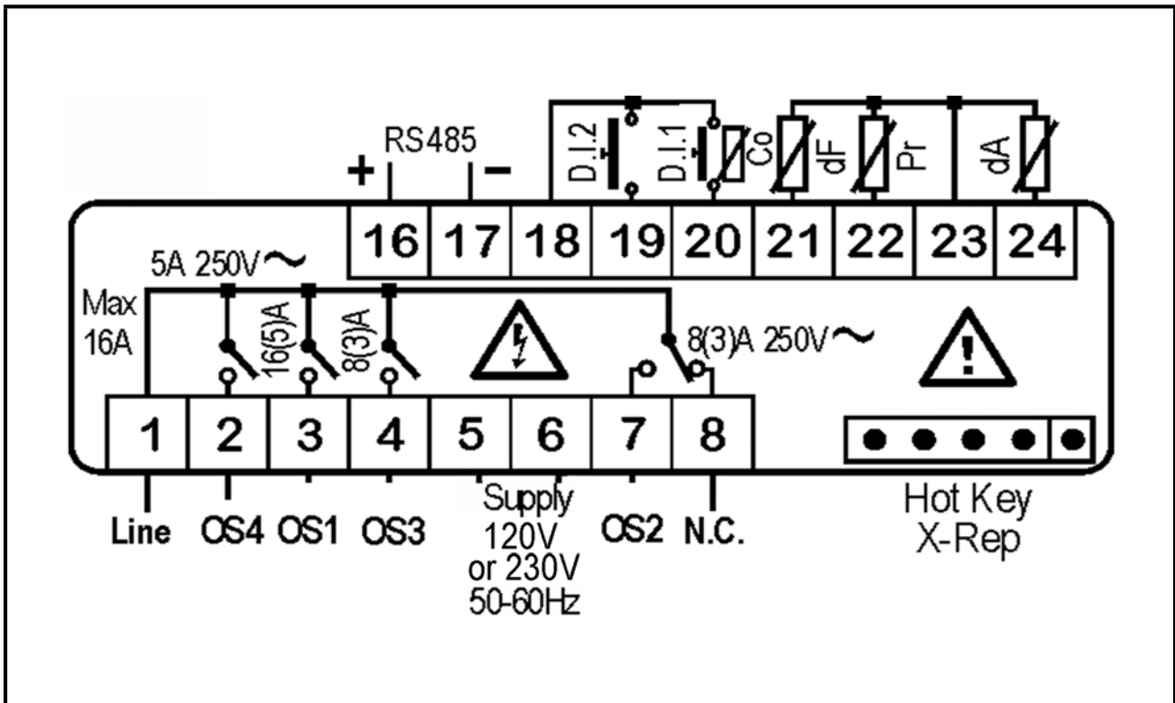
Figure 14-1 - XR75CX-CD Connections
