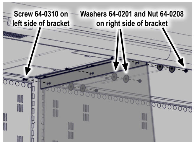
FIGURE 4: Install Plexi Divider Using Washers, Nuts, and Screws
