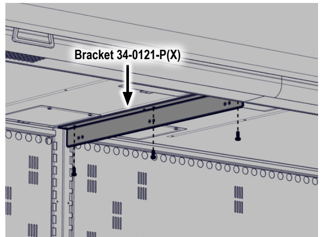
FIGURE 2: Install Bracket Using Screws
