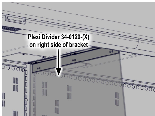
FIGURE 3: Remove Protective Film from Plexi Divider and Then Position It
