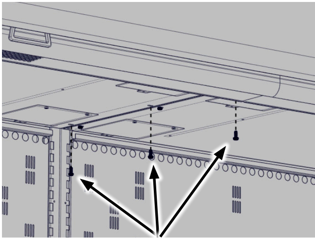
FIGURE 1: Remove Screws from Right Side of Left Case Ceiling
